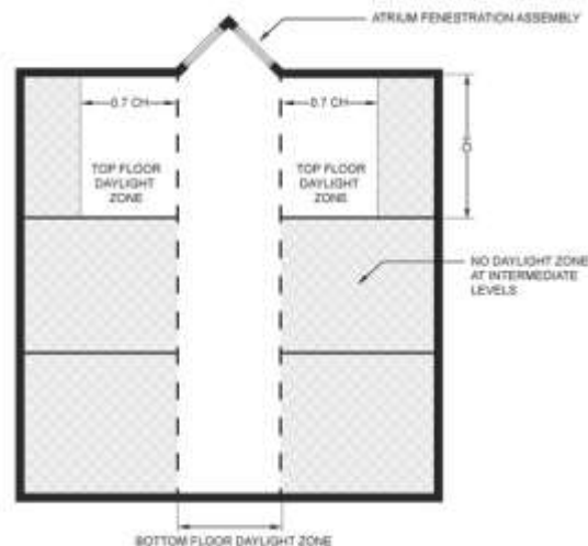
FIGURE C405.2.4.3(24) DAYLIGHT-TOPLIT ZONE UNDER ATRIUM FENESTRATION
