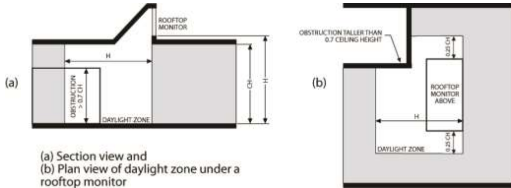
FIGURE C405.2.4.2(3) DAYLIGHT-TOPLIT ZONE UNDER A SLOPED ROOFTOP MONITOR
