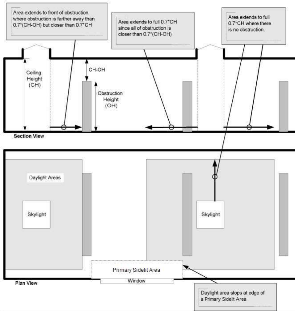
FIGURE C405.2.4.3(1) DAYLIGHT-TOPLIT ZONE UNDER A ROOFTOP FENESTRATION ASSEMBLY
